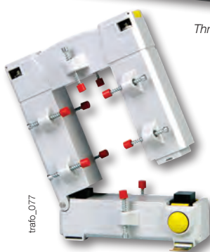
Split-core CT
