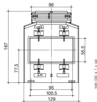
TBA 100 from 600 to 2500 A (1) T2BA 100 from 1200 to 3000 A
